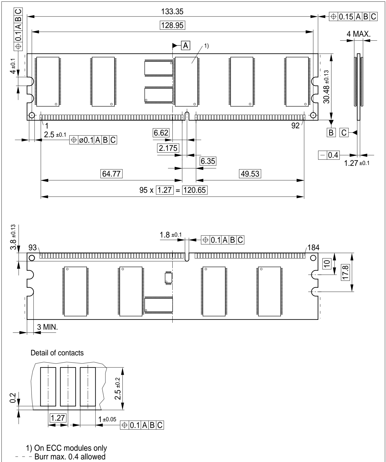
Figure 5 Package Outline RDIMM Raw Card (L-DIM-184-L13-2)
