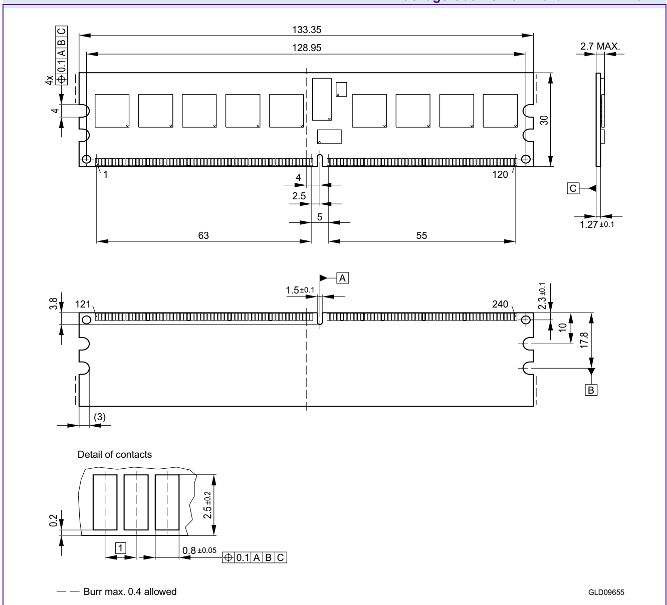
FIGURE 5 Package Outline Raw Card F L-DIM-240-11
