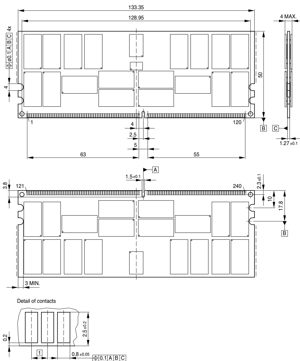
FIGURE 2 Package Outline Raw Card ZZ L-DIM-240-42
