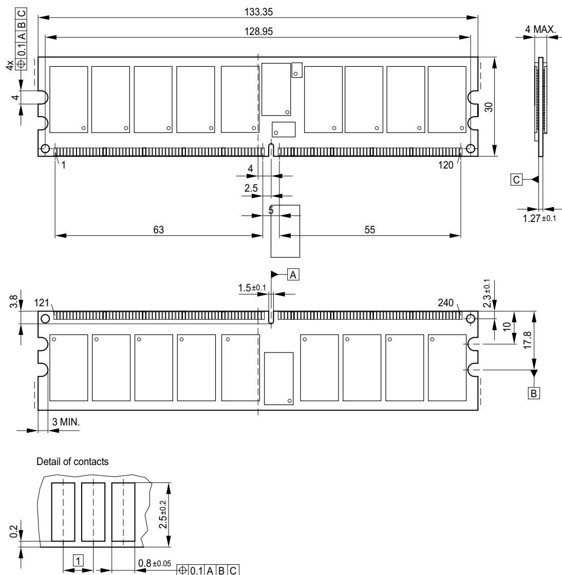
FIGURE 5 Package Outline Raw Card K L-DIM-240-70
