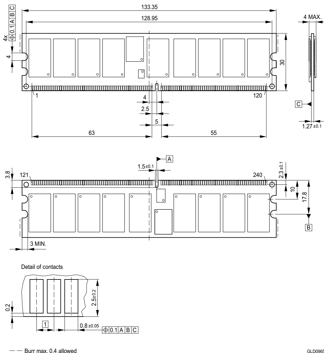
FIGURE 5 Package Outline Raw Card D L-DIM-240-15
