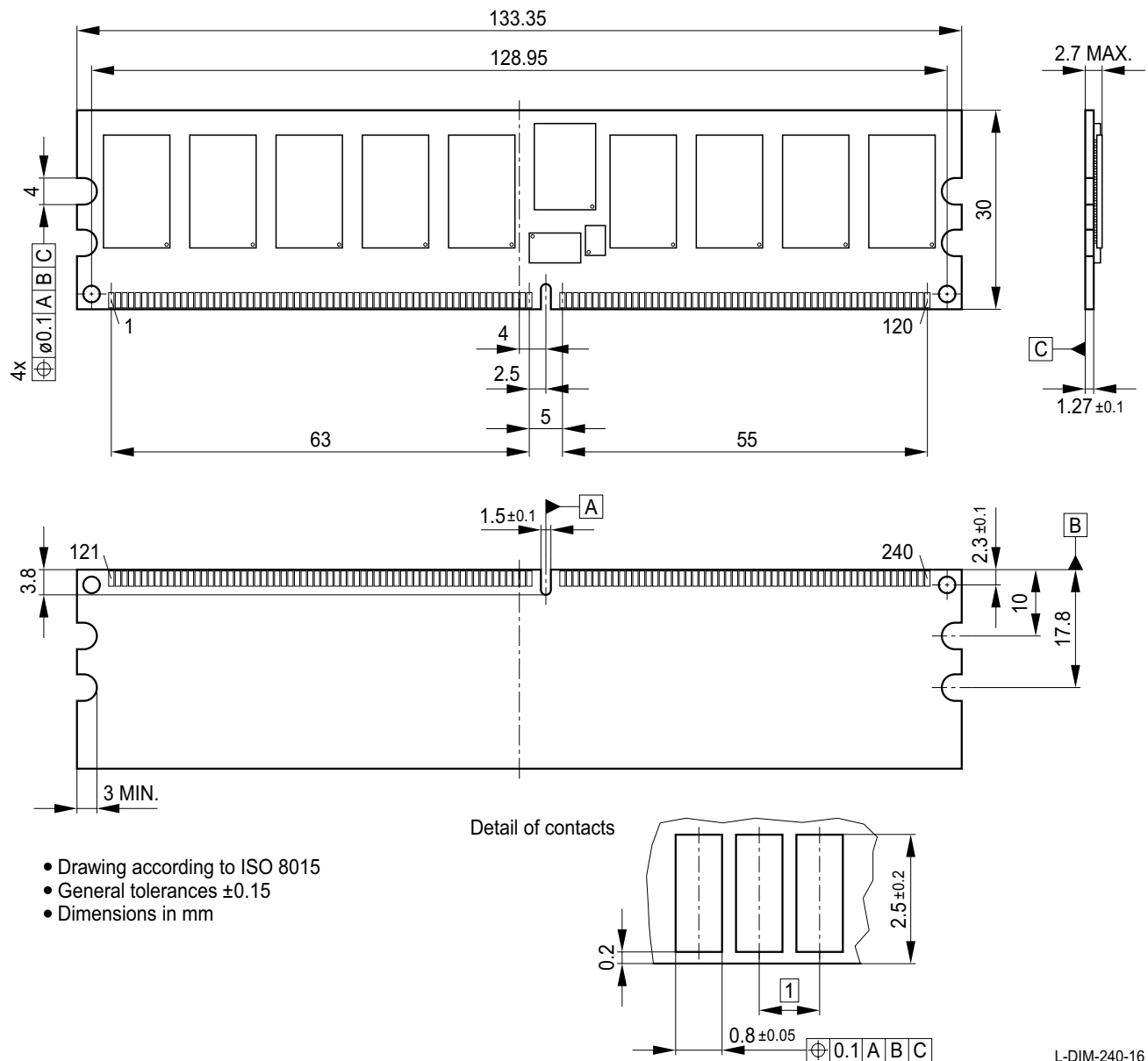
FIGURE 6 Package Outline Raw Card Z L-DIM-240-16
