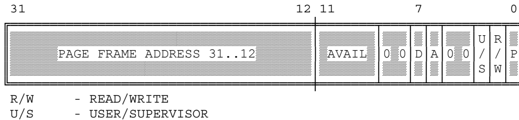
Figure 6-10. Protection Fields of Page Table Entries
