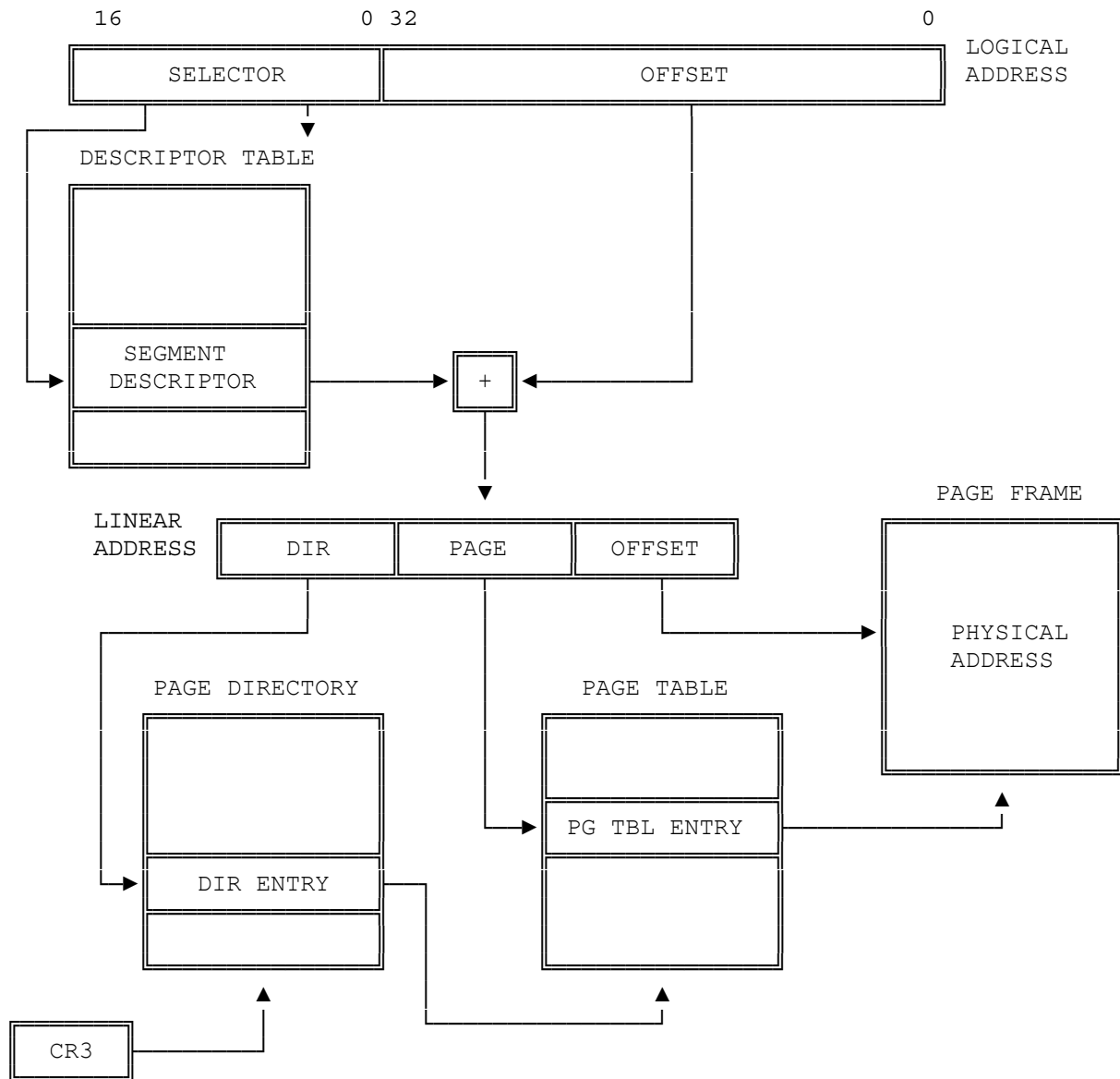
Figure 5-12. 80386 Addressing Mechanism
