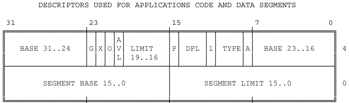
Figure 5-3. General Segment-Descriptor Format
