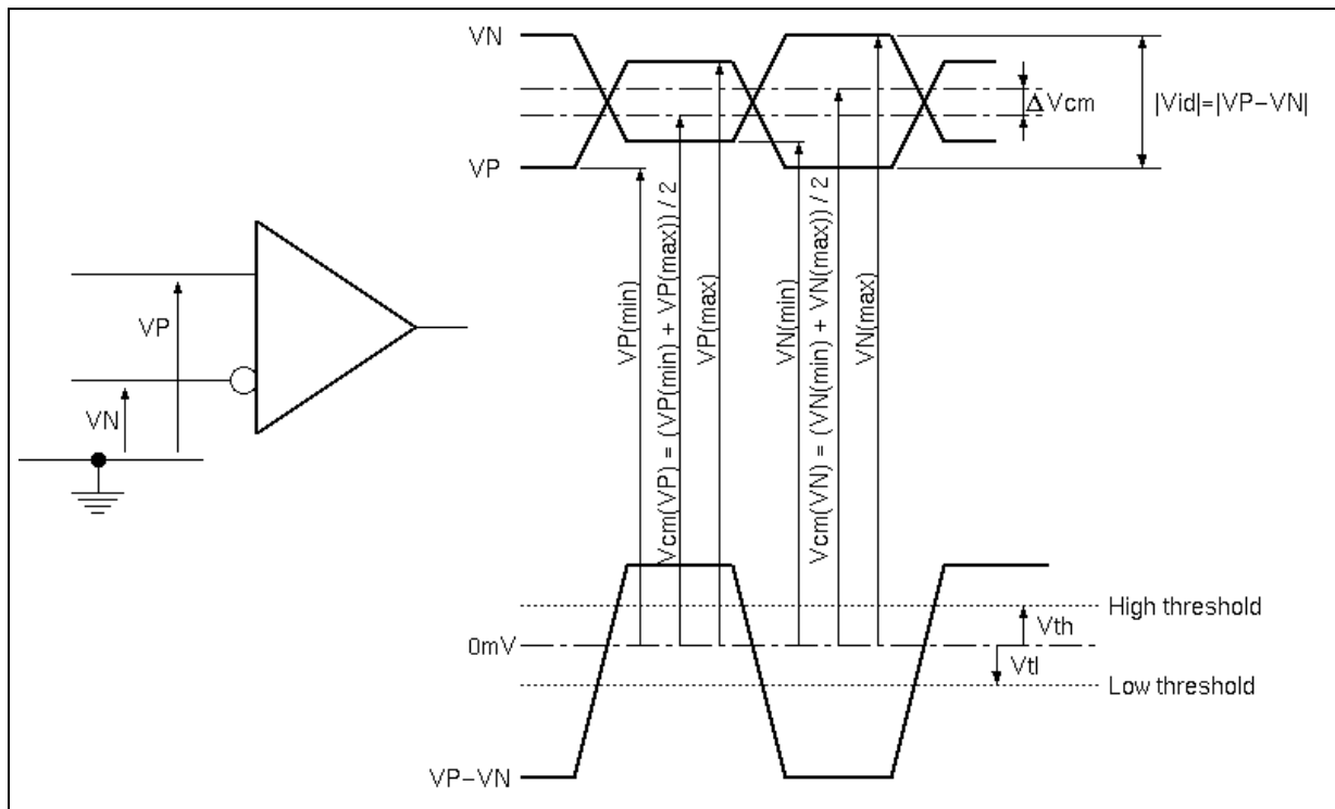
Figure. Voltage Definitions
