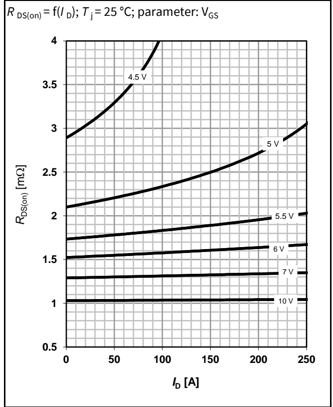
8 Typ. drain-source on-state resistance
