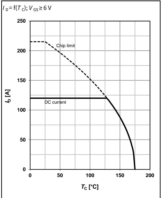
2 Drain current
