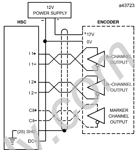
Encoder Wiring in Differential Configuration: Positive Loop
