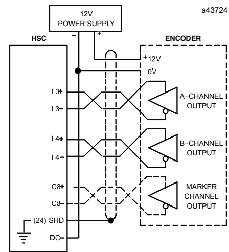
Encoder Wiring in Differential Configuration: Negative Loop
