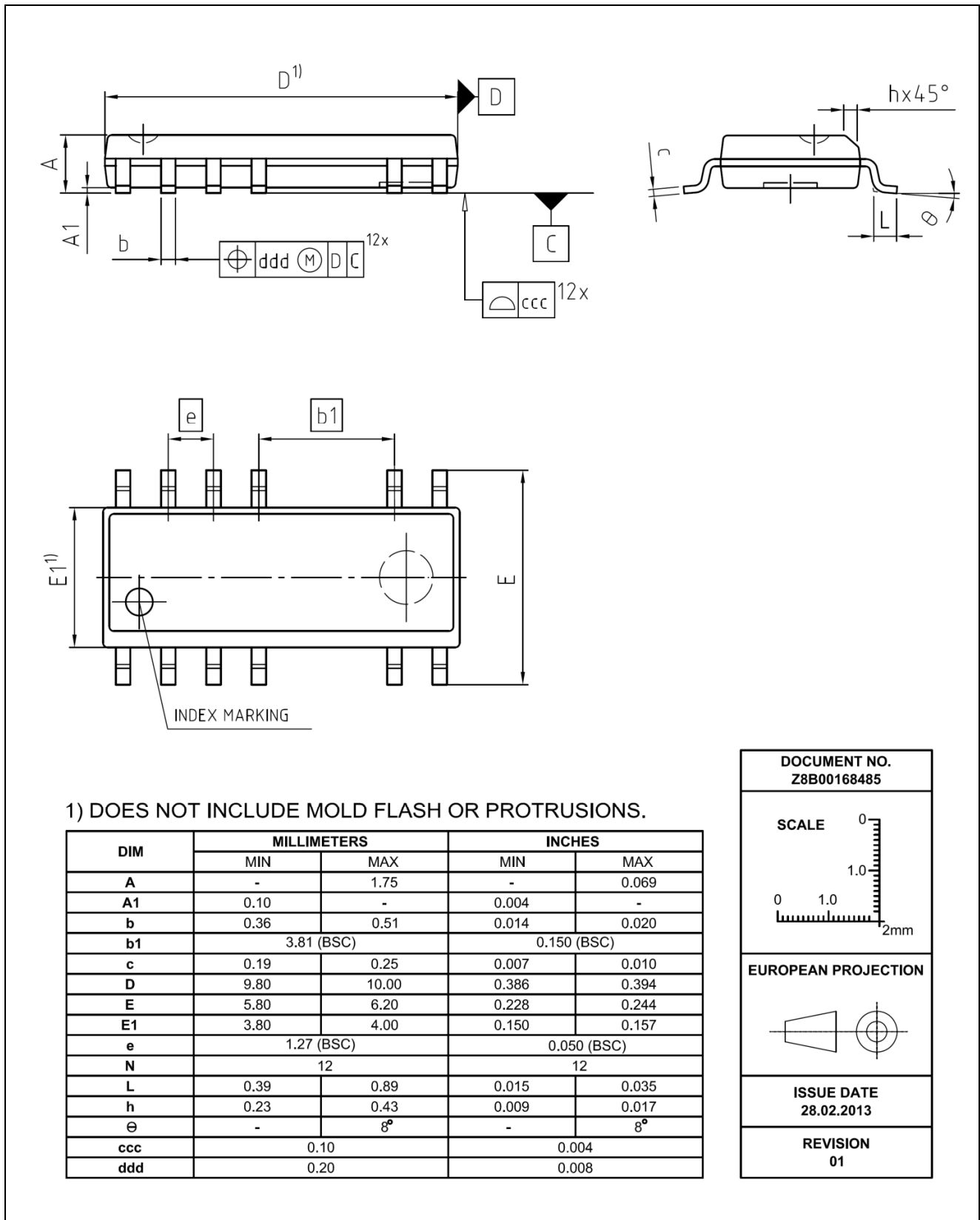
Figure 15 PG-DSO-16/12 (Pb-free lead plating Plastic Dual Small Outline Package)
