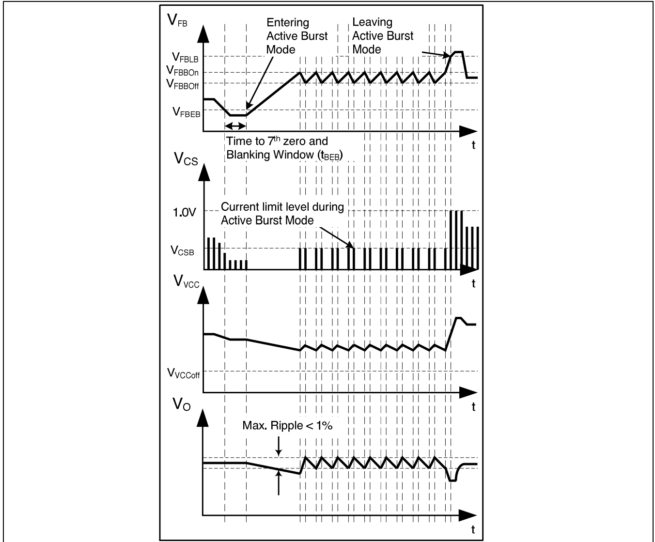
Figure 9 Signals in Active Burst Mode
