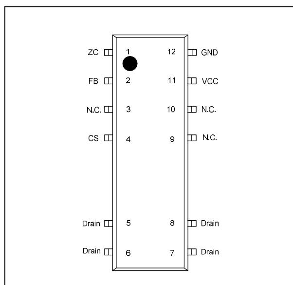
Figure 2 Pin configuration PG-DSO-16/12 (top view)
