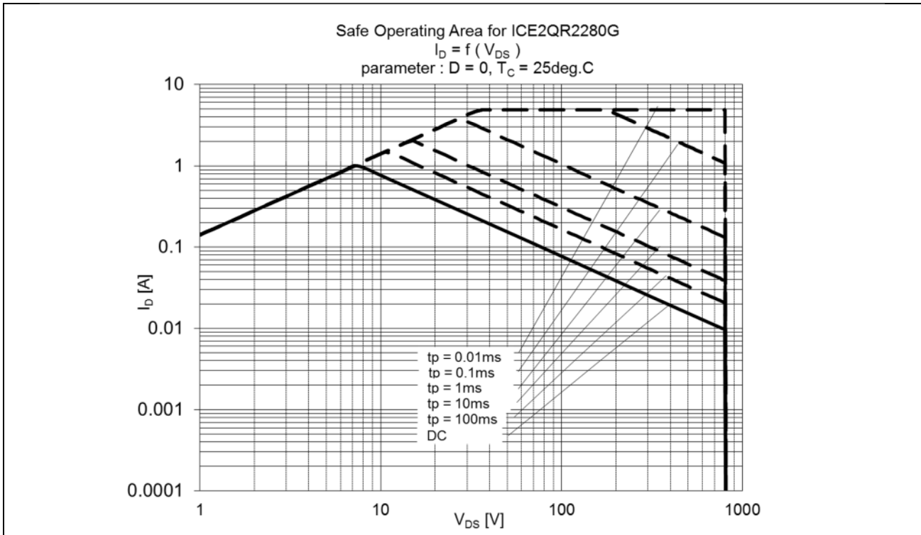
Figure 10 Safe Operating Area (SOA) curve for ICE2QR2280G-1
