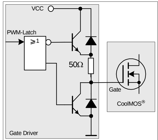
Figure 15 Gate Driver
