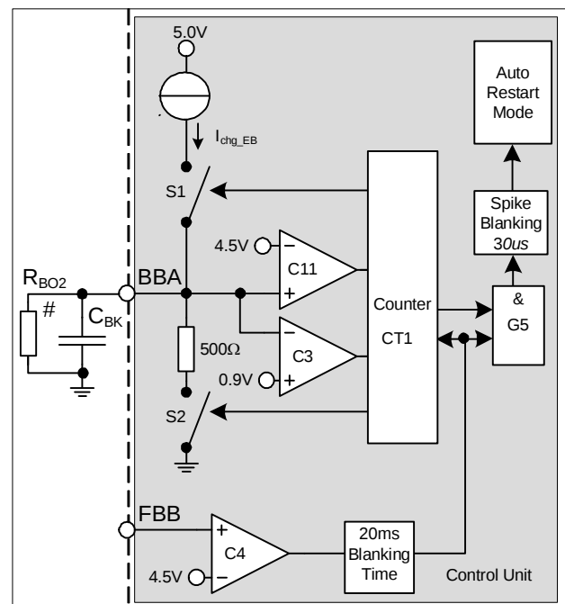
Figure 22 Basic and Extendable Blanking Mode
