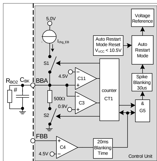
Figure 30 Over load, open loop protection
