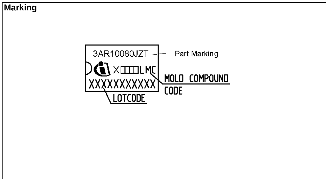
Figure 40 Marking for ICE3AR10080JZ-T
