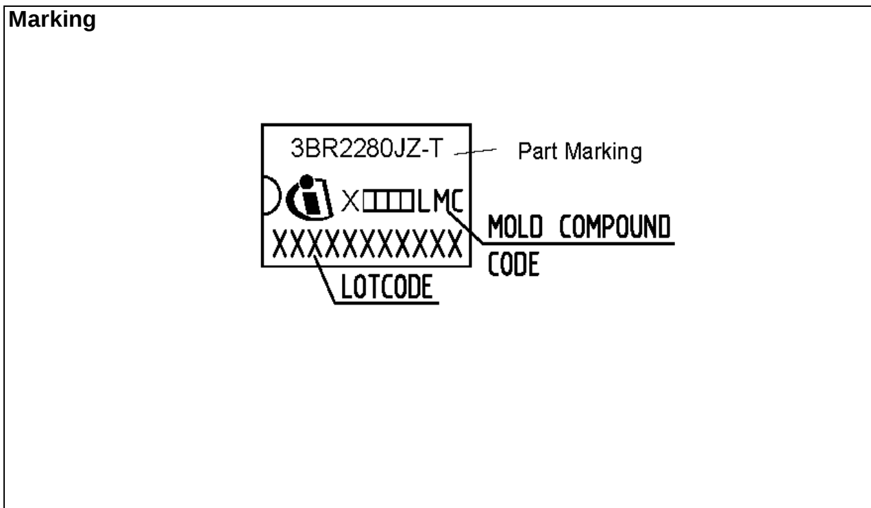
Figure 40 Marking for ICE3BR2280JZ-T
