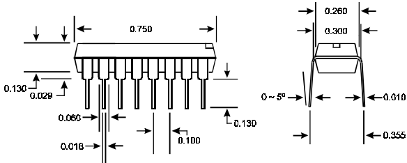
16-Pin DIP Package
