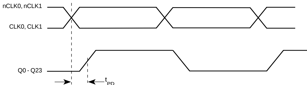
FIGURE 6 - PROPAGATION DELAY
