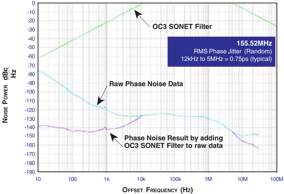
TYPICAL PHASE NOISE AT 155.52MHz At 3.3V
