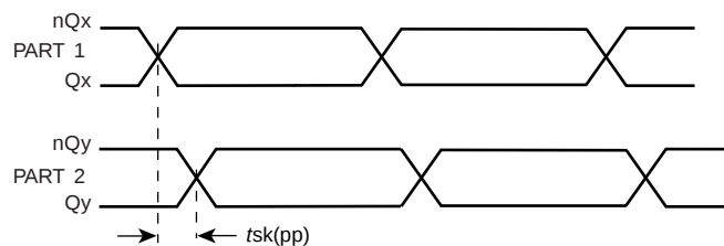
PART-TO-PART SKEW
