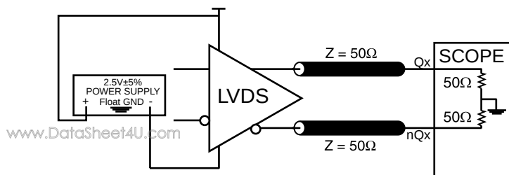
OUTPUT LOAD AC TEST CIRCUIT
