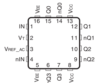
ICS858020 16-Lead VFQFN 3mm x 3mm x 0.95 package body K Package Top View
