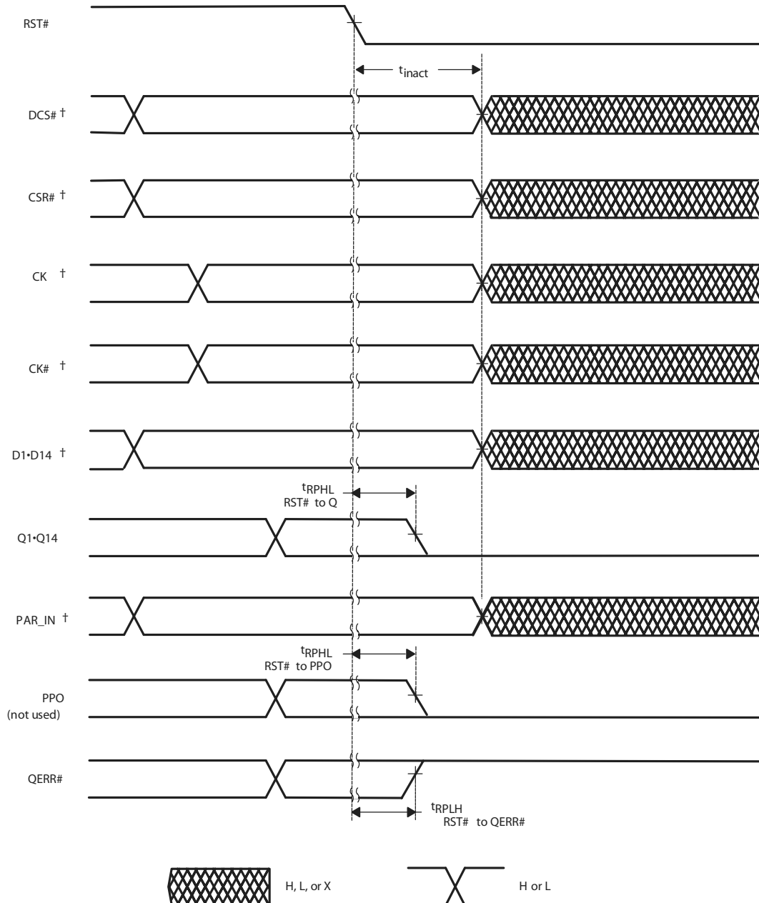
Figure 17 — Timing diagram for the second SSTU32866 (1:2 register-B configuration) device used in pair; C0=1, C1=1; RST# switches from H to L
