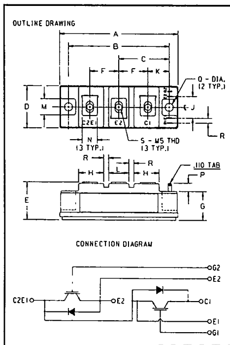
ID226005 Dual IGBTMOD™ Power Module 50 Amperes/600 Volts
