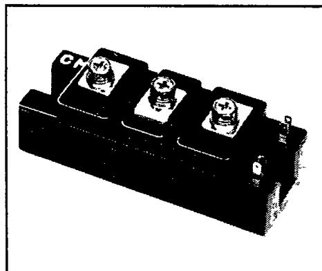
ID226005 Dual IGBTMOD™ Power Module 50 Amperes/600 Volts
