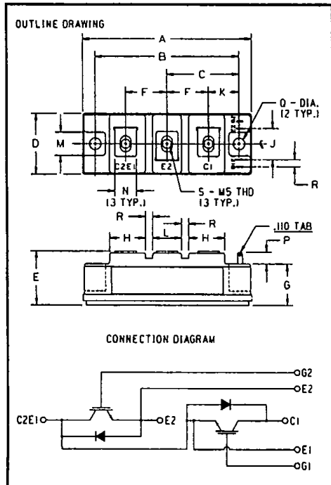
ID226010 Outline Drawing
