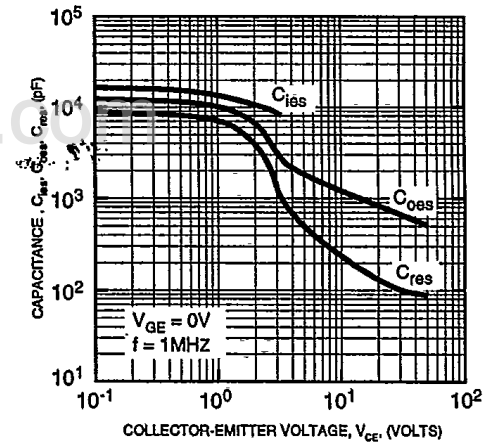
CAPACITANCE VS. V_{CE} (TYPICAL)
