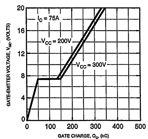
GATE CHARGE, VGE
