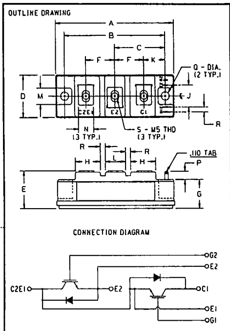
ID226075 Outline Drawing
