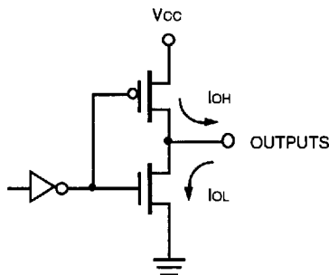
Figure 3. Output Structure
