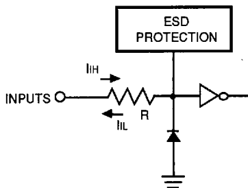
Figure 2. Input Structure
