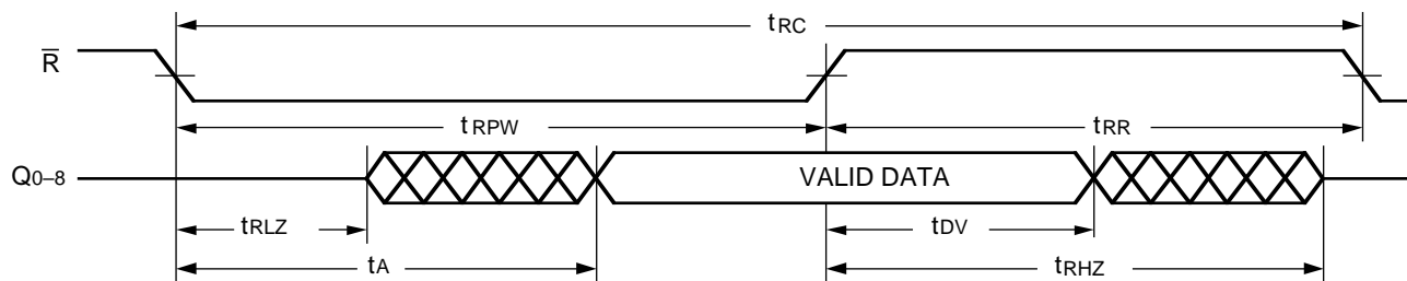
Figure 3. Read Operation
