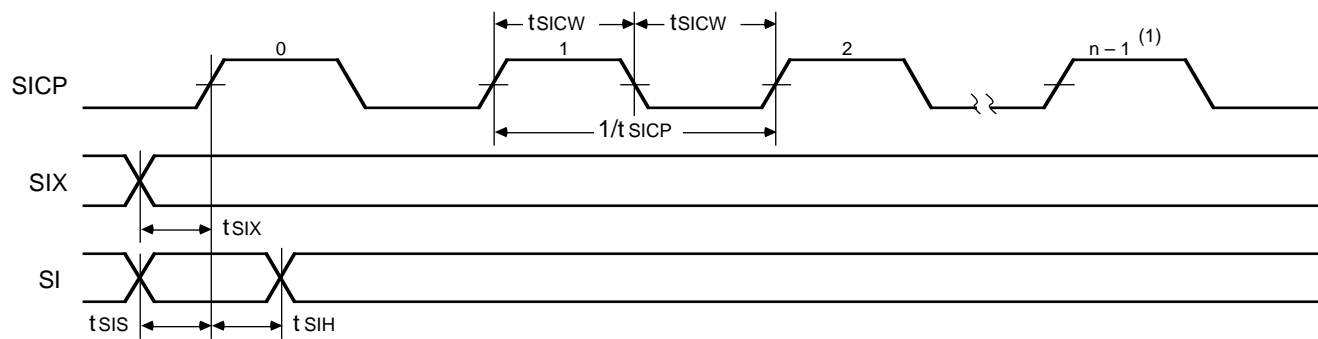
Figure 2. Write Operation
