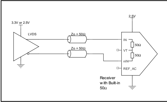
Figure 5A. IN/nIN Input with Built-In 50Ω Driven by an LVDS Driver
