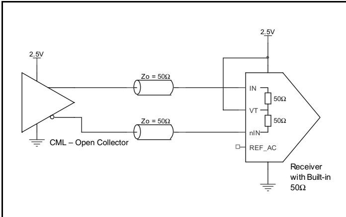
Figure 5C. IN/nIN Input with Built-In 50Ω Driven by a CML Driver
