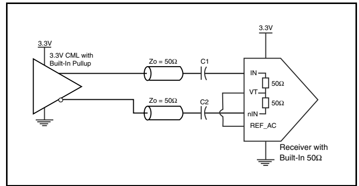
Figure 4D. IN/nIN Input with Built-In 50Ω Driven by a CML Driver with Built-In 50Ω Pullup
