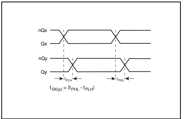
Pulse Skew
