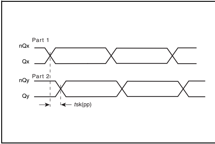
Part-to-Part Skew
