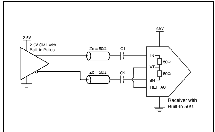
Figure 5D. IN/nIN Input with Built-In 50Ω Driven by a CML Driver with Built-In 50Ω Pullup
