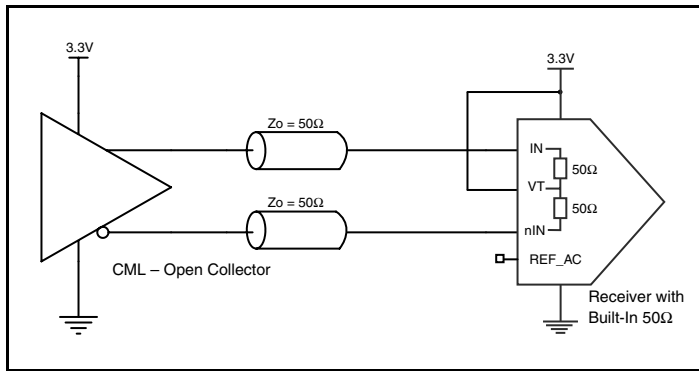
Figure 4C. IN/nIN Input with Built-In 50Ω Driven by a CML Driver
