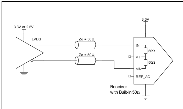
Figure 4A. N/nIN Input with Built-In 50Ω Driven by an LVDS Driver
