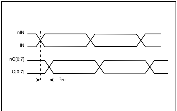
Propagation Delay
