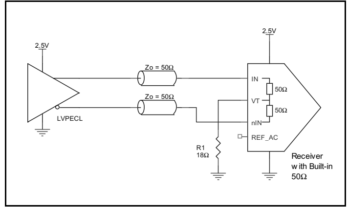
Figure 5B. IN/nIN Input with Built-In 50Ω Driven by an LVPECL Driver
