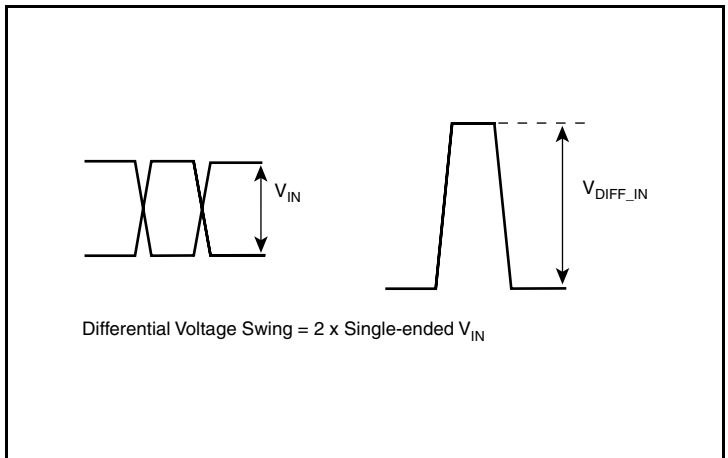
Single-Ended & Differential Input, Output Voltage Swing
