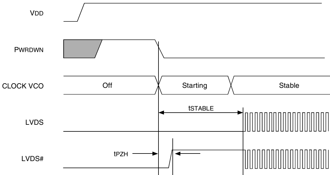
PWRDWN De-Assertion
