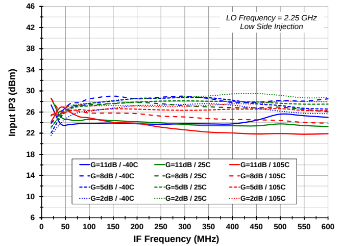
Input IP3 vs. Temperature and Gain Setting (LO=2.25 GHz)
