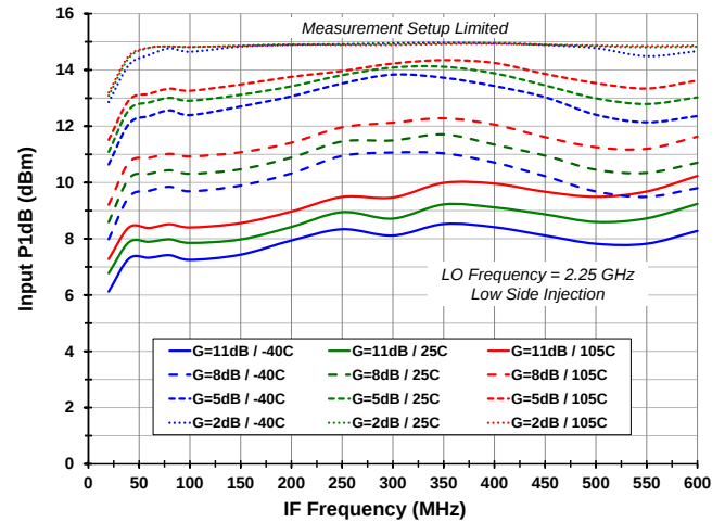
Input P1dB vs. Temperature and Gain Setting (LO=2.25 GHz)
