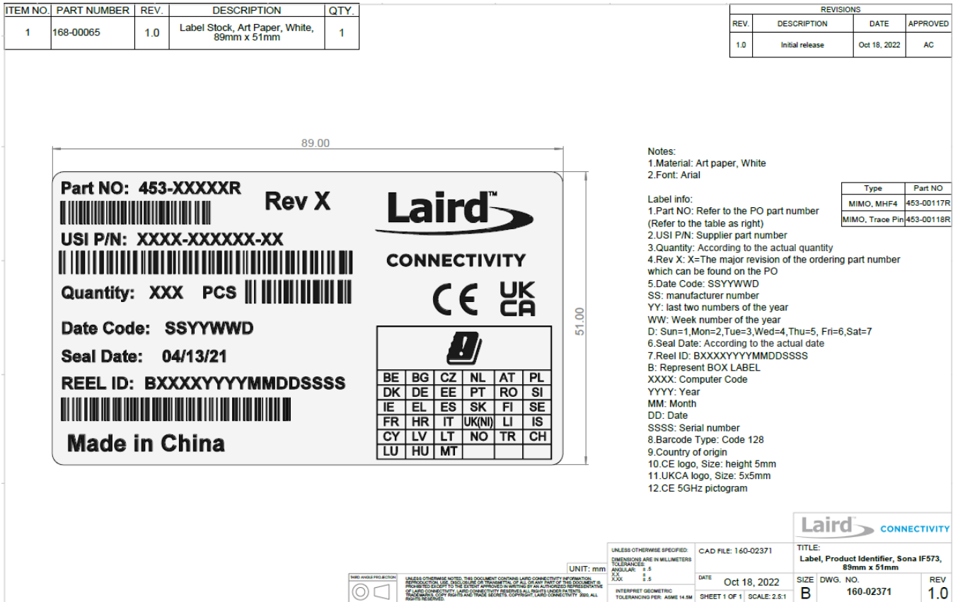
Figure 29: Sona IF573 Bag and Box Product Identifier Label, 160-02371
