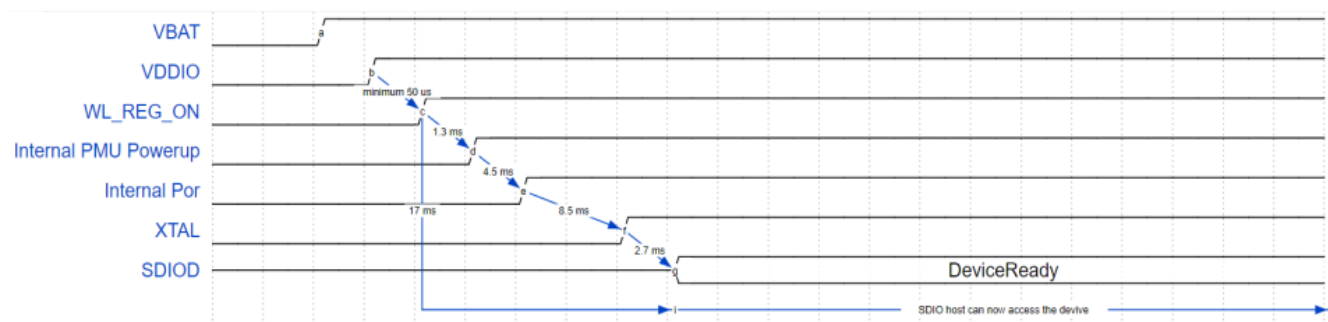
Figure 19: WLAN Boot-Up Sequence for SDIO Host
