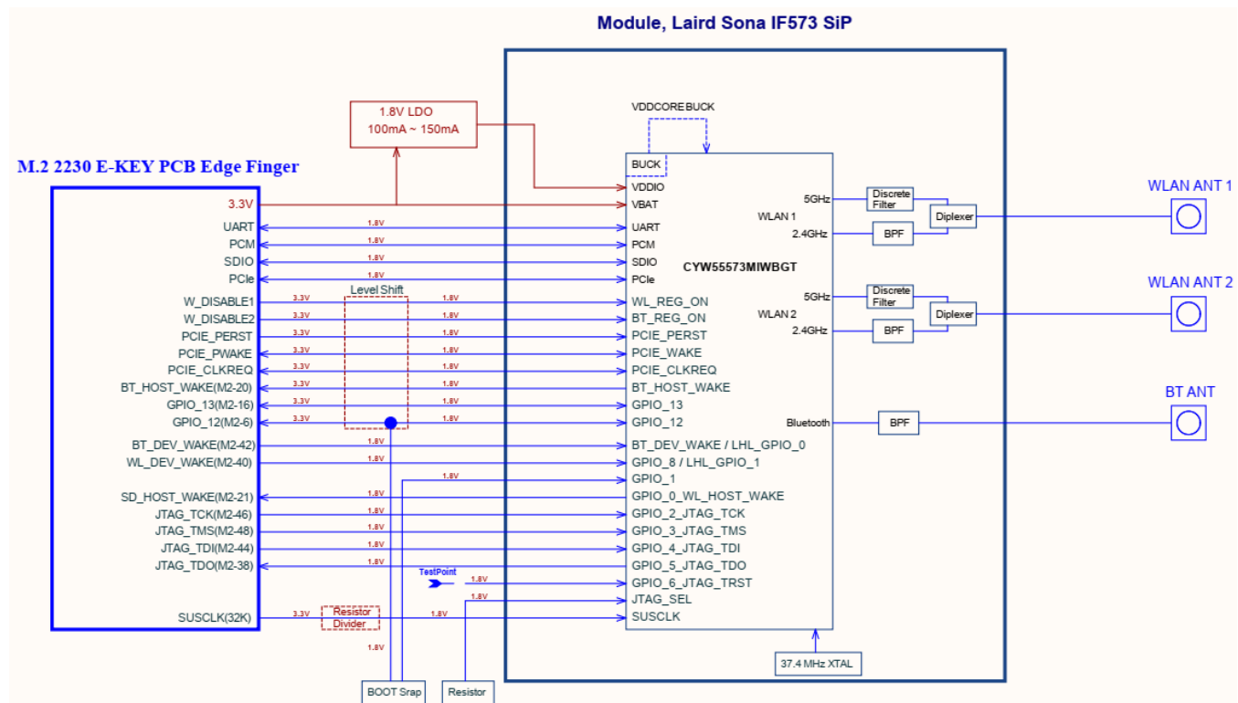
Figure 2: M.2 2230 E-Key
