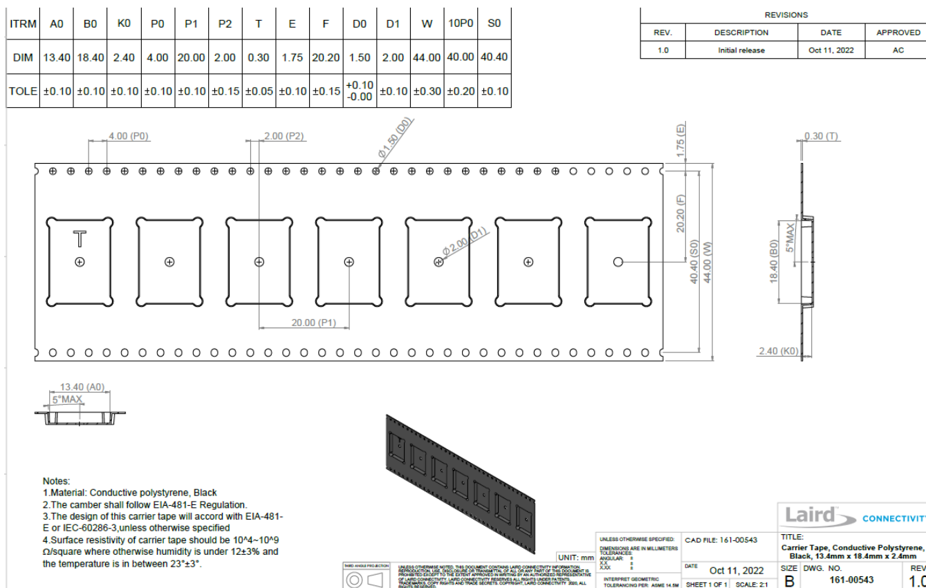
Figure 26: Sona IF573 Tape specifications, 161-00543
