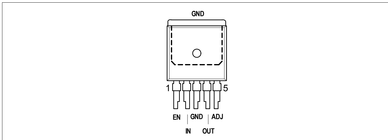
Figure 2 Pin Configuration PG-T0263-5
