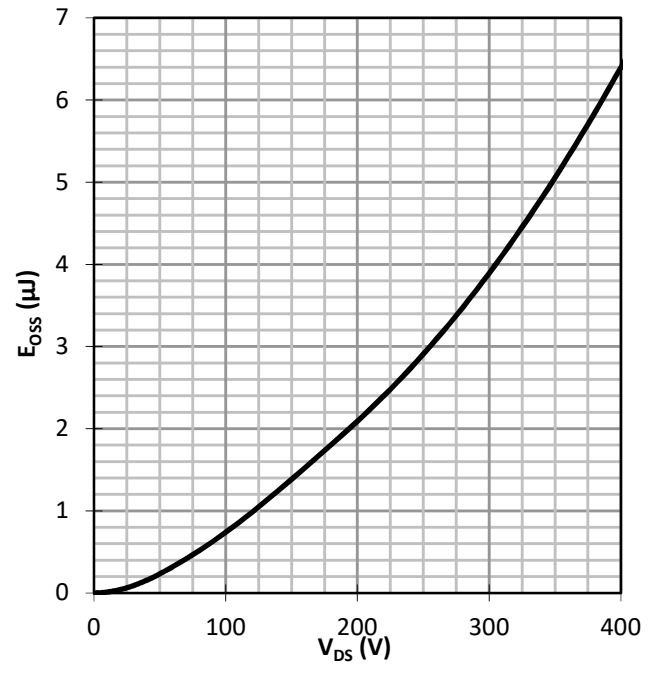
Figure 20 Typ. Coss stored Energy
