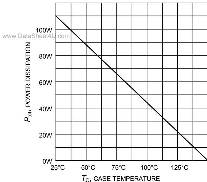
Figure 3. Power dissipation as a function of case temperature ( T_j \leq 150^\circ\text{C} )
