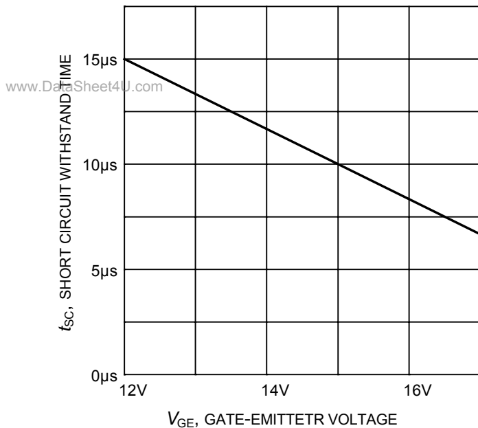
Figure 19. Short circuit withstand time as a function of gate-emitter voltage ( V_{CE}=600V, \text{start at } T_j=25^\circ\text{C} )
