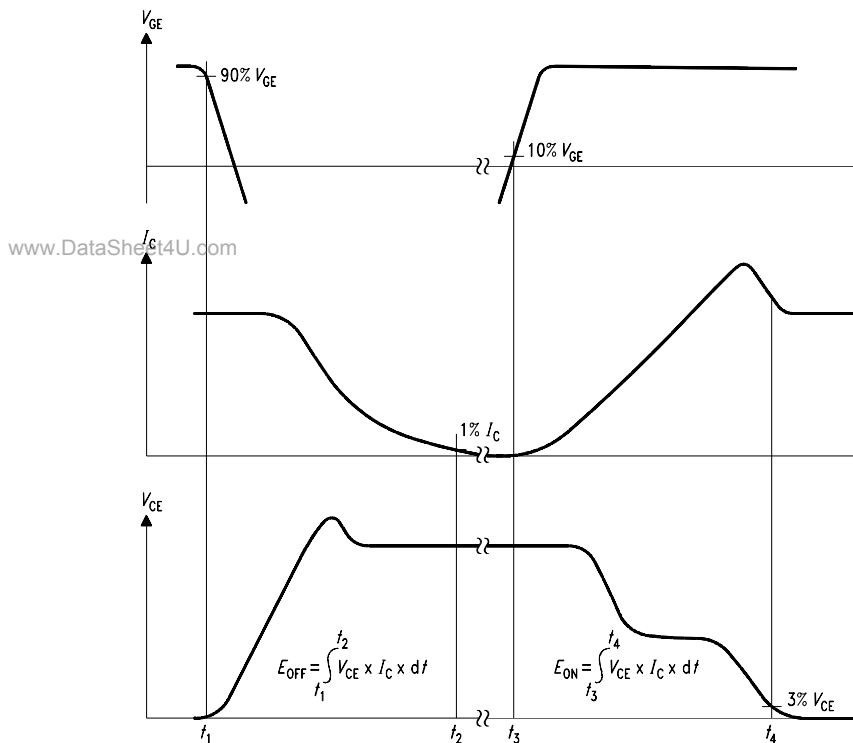
Figure B. Definition of switching losses
