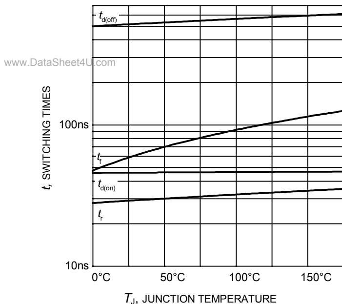
Figure 11. Typical switching times as a function of junction temperature (inductive load, V_{CE}=600\text{V} , V_{GE}=0/15\text{V} , I_C=15\text{A} , R_G=56\Omega , Dynamic test circuit in Figure E)
