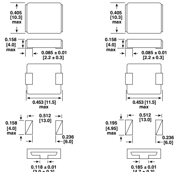
The diagram above applies to values 1.8 \mu\text{H} and above.
