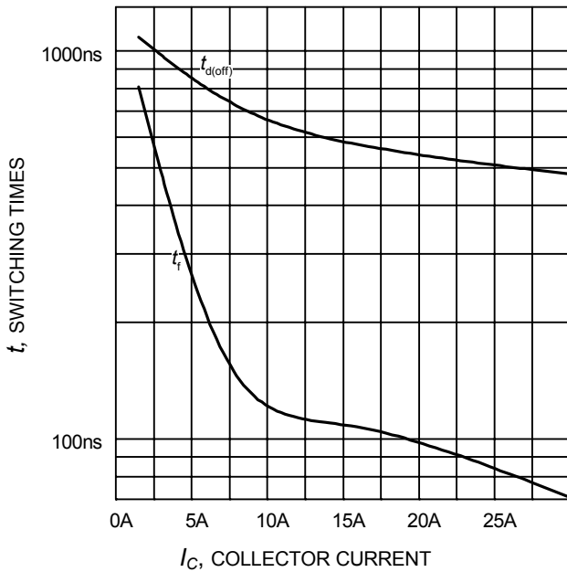
Figure 9. Typical switching times as a function of collector current (inductive load, T_J=175^{\circ}\text{C} , V_{CE}=600\text{V} , V_{GE}=0/15\text{V} , R_G=54\Omega , Dynamic test circuit in Figure E)
