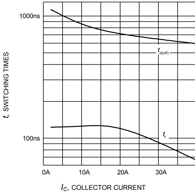
Figure 9. Typical switching times as a function of collector current (inductive load, T_J=175^{\circ}\text{C} , V_{CE}=600\text{V} , V_{GE}=0/15\text{V} , R_G=47\Omega , Dynamic test circuit in Figure E)
