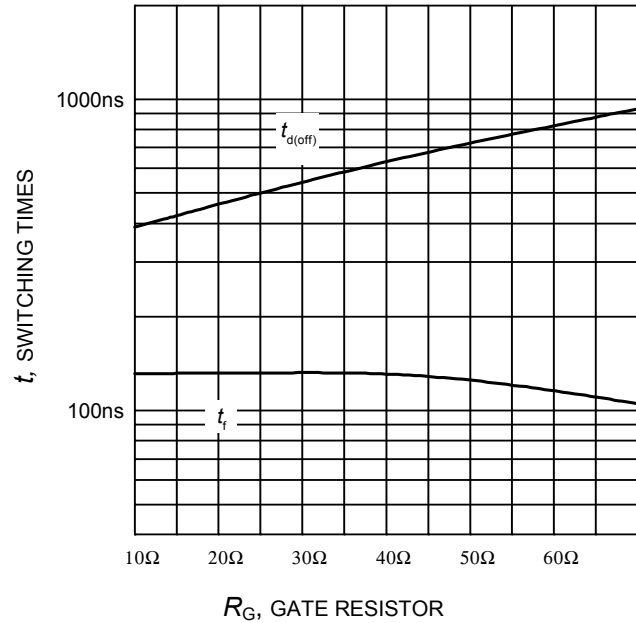
Figure 10. Typical switching times as a function of gate resistor (inductive load, T_J=175^{\circ}\text{C} , V_{CE}=600\text{V} , V_{GE}=0/15\text{V} , I_C=20\text{A} , Dynamic test circuit in Figure E)
