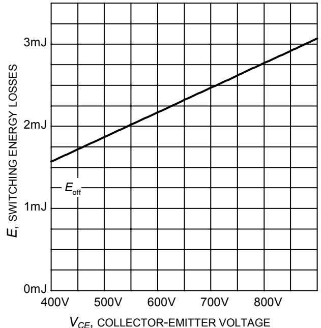
Figure 16. Typical turn-off energy as a function of collector emitter voltage (inductive load, T_J=175^\circ\text{C} , V_{GE}=0/15\text{V} , I_C=20\text{A} , R_G=29\Omega , Dynamic test circuit in Figure E)
