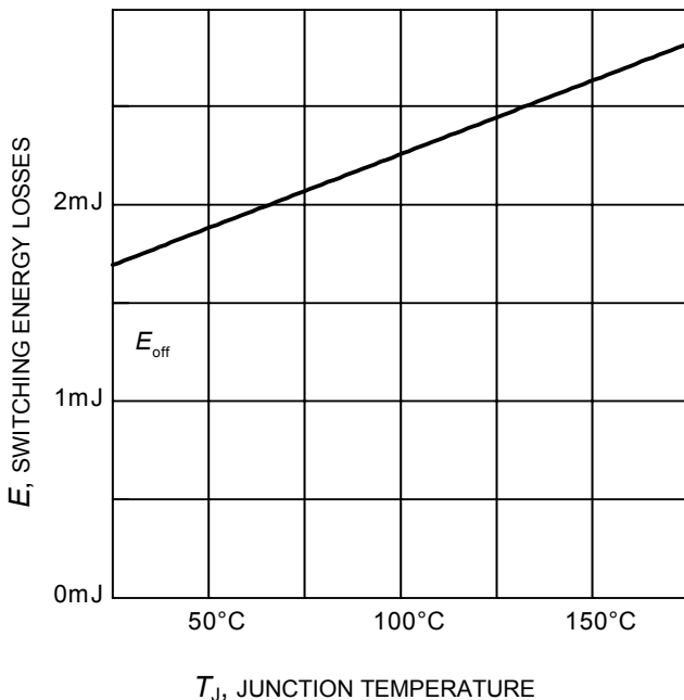
Figure 15. Typical turn-off energy as a function of junction temperature (inductive load, V_{CE}=600\text{V} , V_{GE}=0/15\text{V} , I_C=20\text{A} , R_G=29\Omega , Dynamic test circuit in Figure E)
