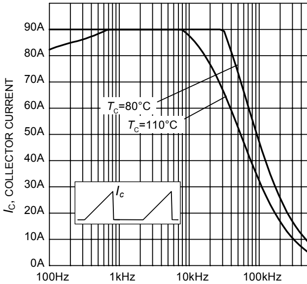
f , SWITCHING FREQUENCY
