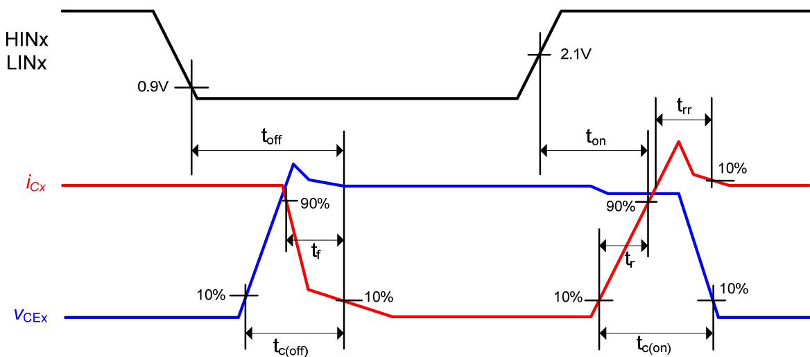
Figure 9: Switching times definition
