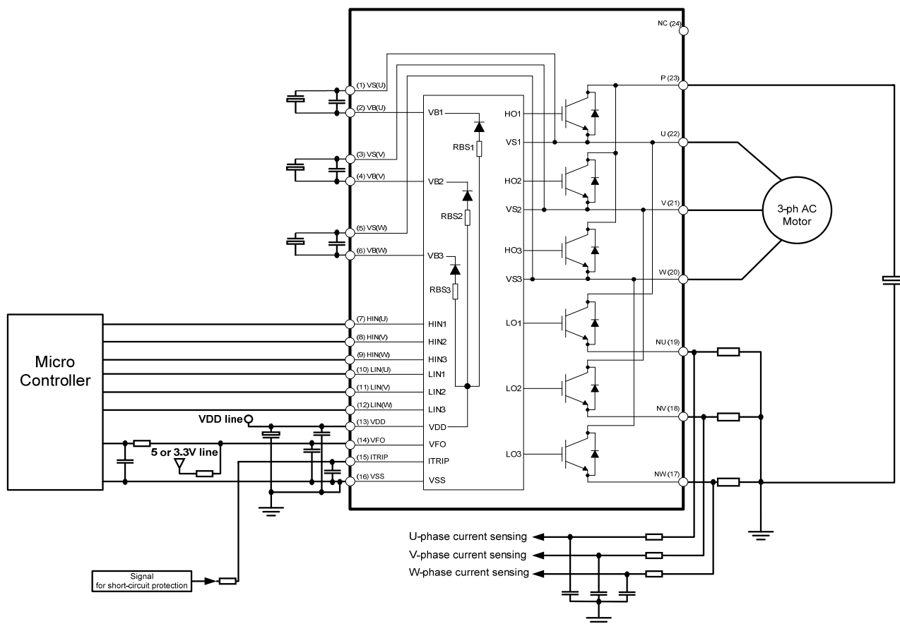
Figure 8: Application circuit
