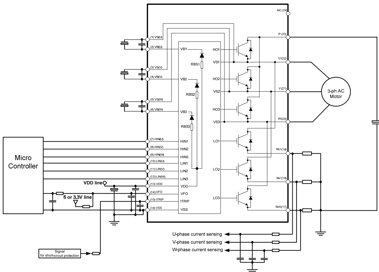
Figure 8: Application circuit
