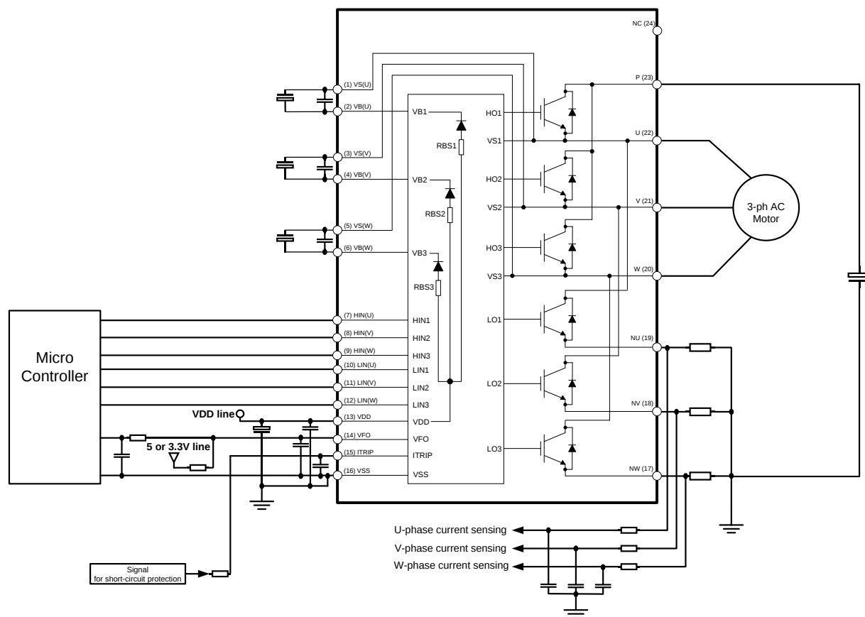
Figure 8: Application circuit
