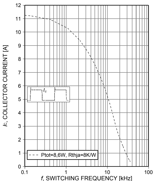
Figure 1. Collector current as a function of switching frequency ( T_{vj} \leq 175^\circ\text{C} , T_a = 55^\circ\text{C} , D = 0.5 , V_{CE} = 400\text{V} , V_{GE} = 15/0\text{V} , r_{g} = 15\Omega , PCB mounting with thermal vias and heatsink, see Appnote: www.infineon.com/igbt )
