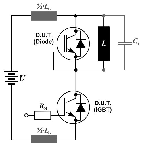
Figure E. Dynamic test circuit Leakage inductance L_\sigma = 180\text{nH} and Stray capacitance C_\sigma = 39\text{pF} .
