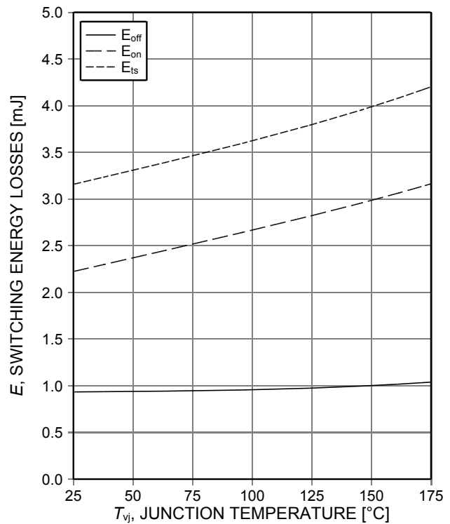
Figure 14. Typical switching energy losses as a function of junction temperature (inductive load, V_{CE}=400\text{V} , V_{GE}=0/15\text{V} , I_C=75\text{A} , R_{G(on)}=8\Omega , R_{G(off)}=8\Omega , dynamic test circuit in Figure E)
