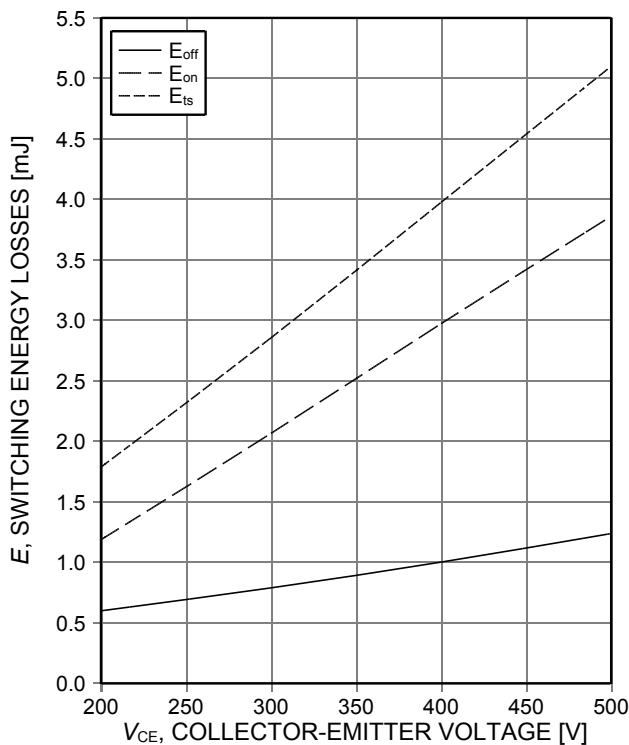
Figure 15. Typical switching energy losses as a function of collector emitter voltage (inductive load, T_{vj}=150^{\circ}\text{C} , V_{GE}=0/15\text{V} , I_C=75\text{A} , R_{G(on)}=8\Omega , R_{G(off)}=8\Omega , dynamic test circuit in Figure E)
