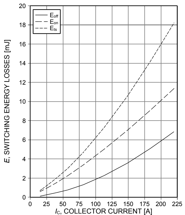
Figure 12. Typical switching energy losses as a function of collector current (inductive load, T_{vj}=150^{\circ}\text{C} , V_{CE}=400\text{V} , V_{GE}=0/15\text{V} , R_{G(on)}=8\Omega , R_{G(off)}=8\Omega , dynamic test circuit in Figure E)
