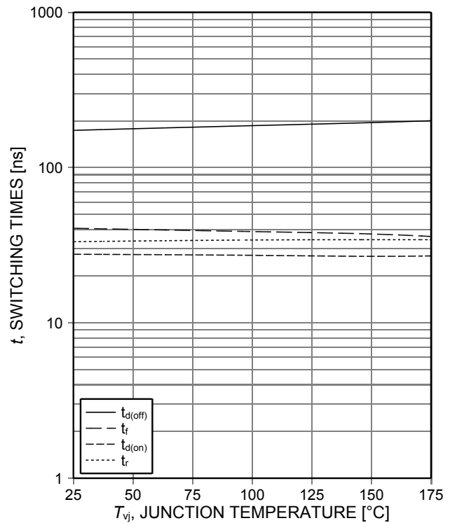
Figure 10. Typical switching times as a function of junction temperature (inductive load, V_{CE}=400\text{V} , V_{GE}=0/15\text{V} , I_C=75\text{A} , R_{G(on)}=8\Omega , R_{G(off)}=8\Omega , dynamic test circuit in Figure E)
