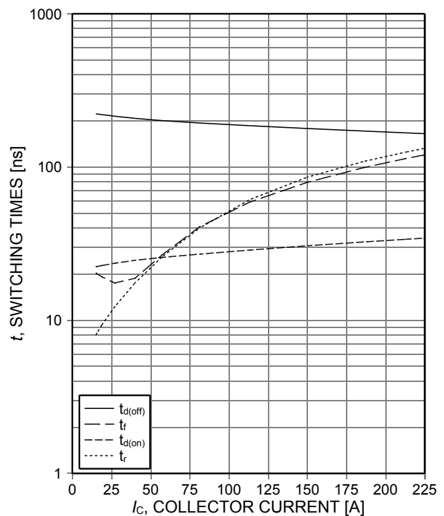
Figure 8. Typical switching times as a function of collector current (inductive load, T_{vj}=150^{\circ}\text{C} , V_{CE}=400\text{V} , V_{GE}=0/15\text{V} , R_{G(on)}=8\Omega , R_{G(off)}=8\Omega , dynamic test circuit in Figure E)
