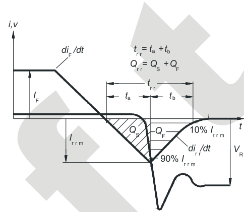
Figure C. Definition of diodes switching characteristics
