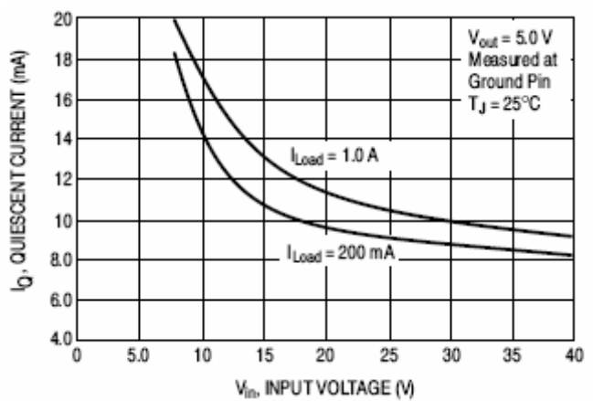
Figure 7. Quiescent Current
