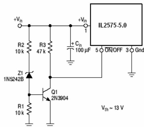
NOTE: This picture does not show the complete circuit. Figure 21. Undervoltage Lockout Circuit for Buck Converter
