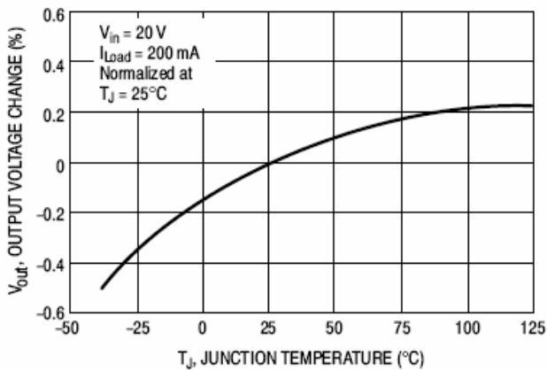
www.DataSheet4U.com Figure 2. Normalized Output Voltage
