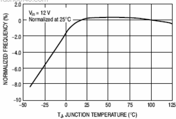
Figure 10. Oscillator Frequency
