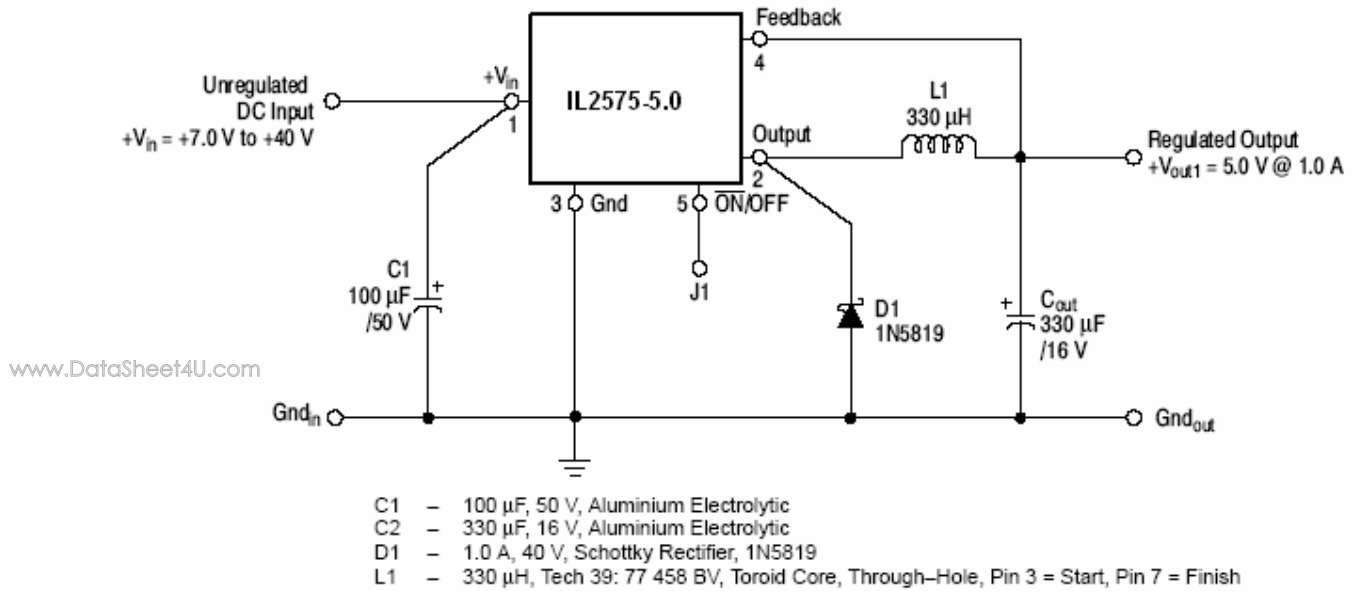
Figure 25. Schematic Diagram of the IL2575-5.0 Step-Down Converter
