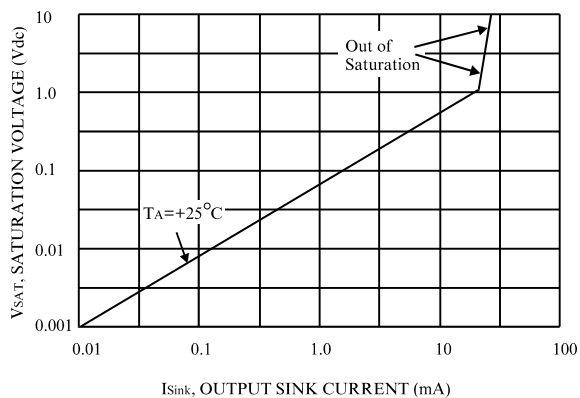
Figure 2. Output Saturation Voltage versus Output Sink Current
