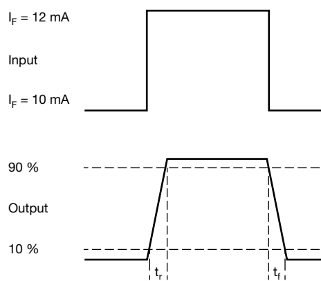
Fig. 2 - Switching Times
