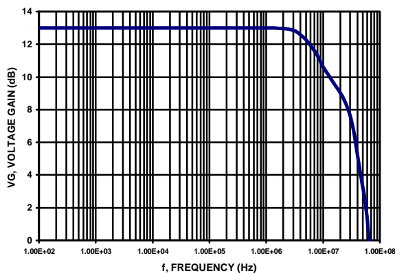
Figure5 . Frequency Response
