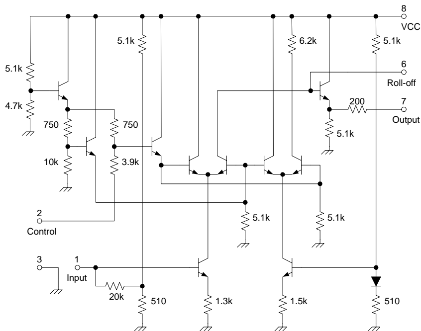
Figure 2. Circuit Schematic
