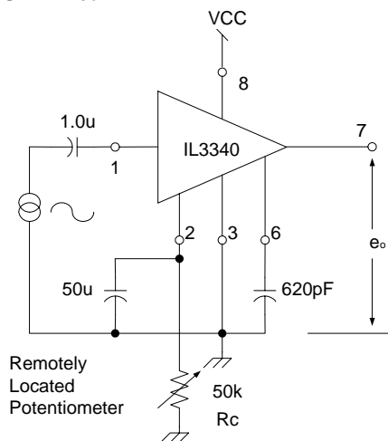
Figure 1. Typical DC Remote Volume Control
