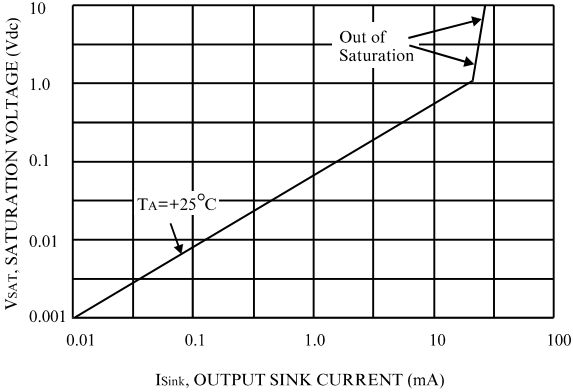
Figure 2. Output Saturation Voltage versus Output Sink Current
