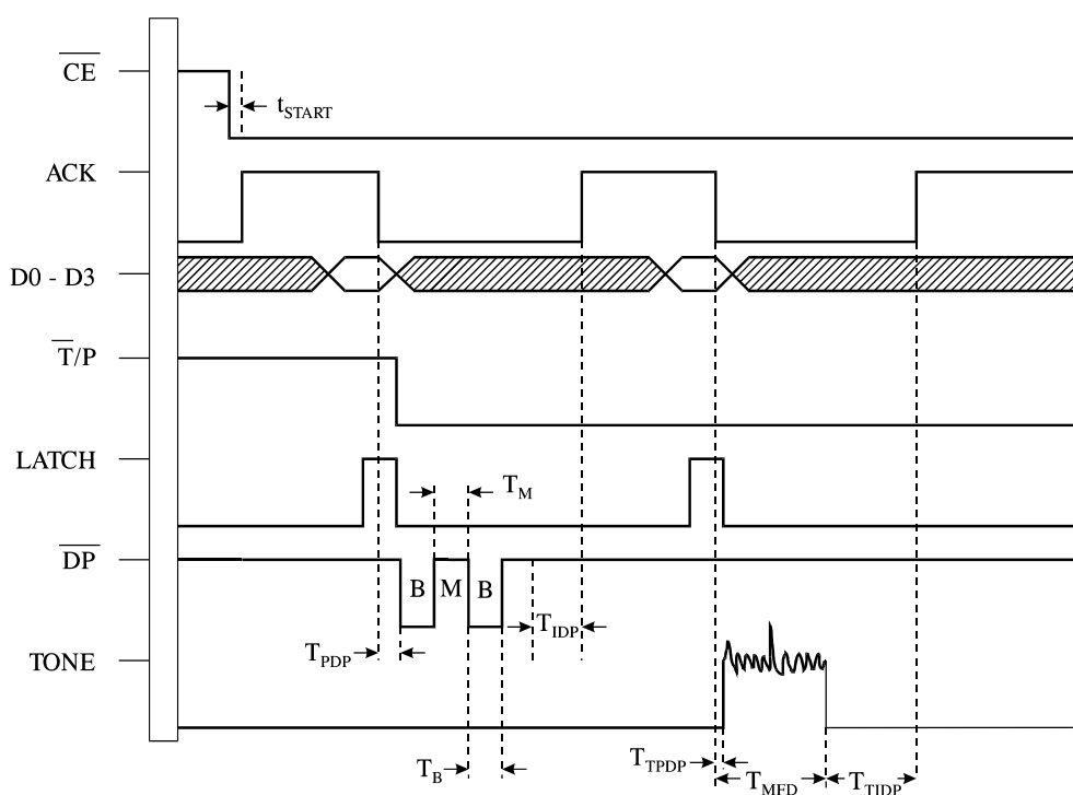
Figure 1. Switching diagram
