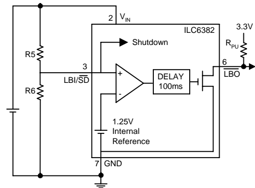
Figure 6: Low Battery Detector
