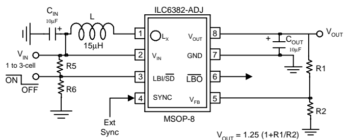
Figure 2: ILC6382-Adj
