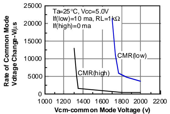
Figure 15. Common mode transient rejection
